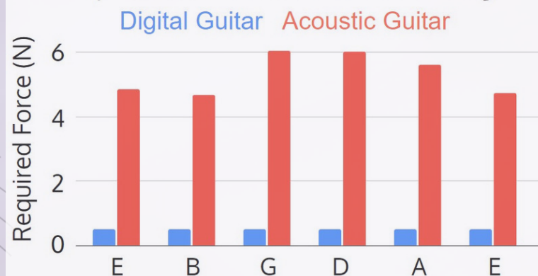
Required Force to Fret Guitar Per String
